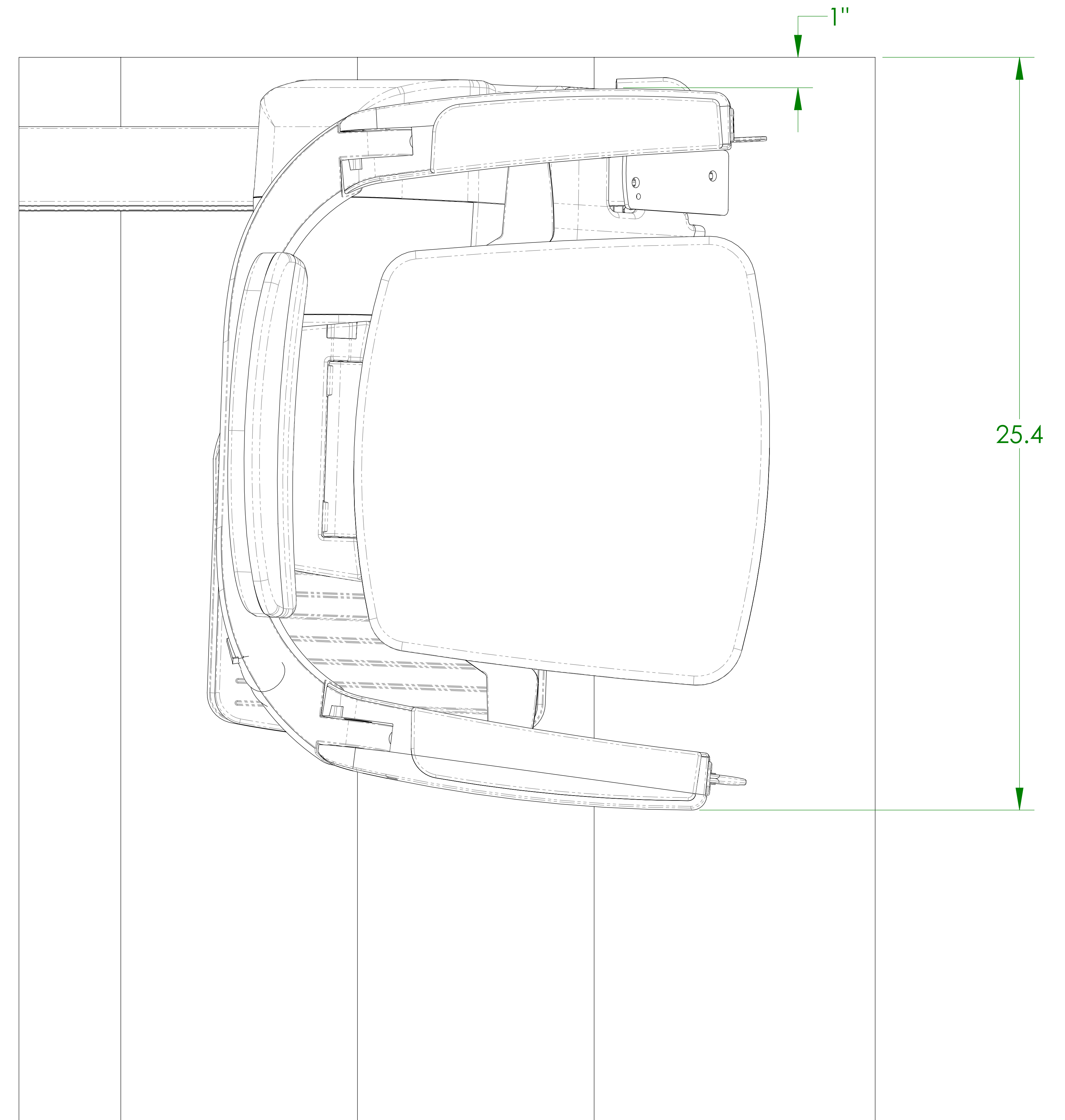
SEAT SWIVELED 90°
