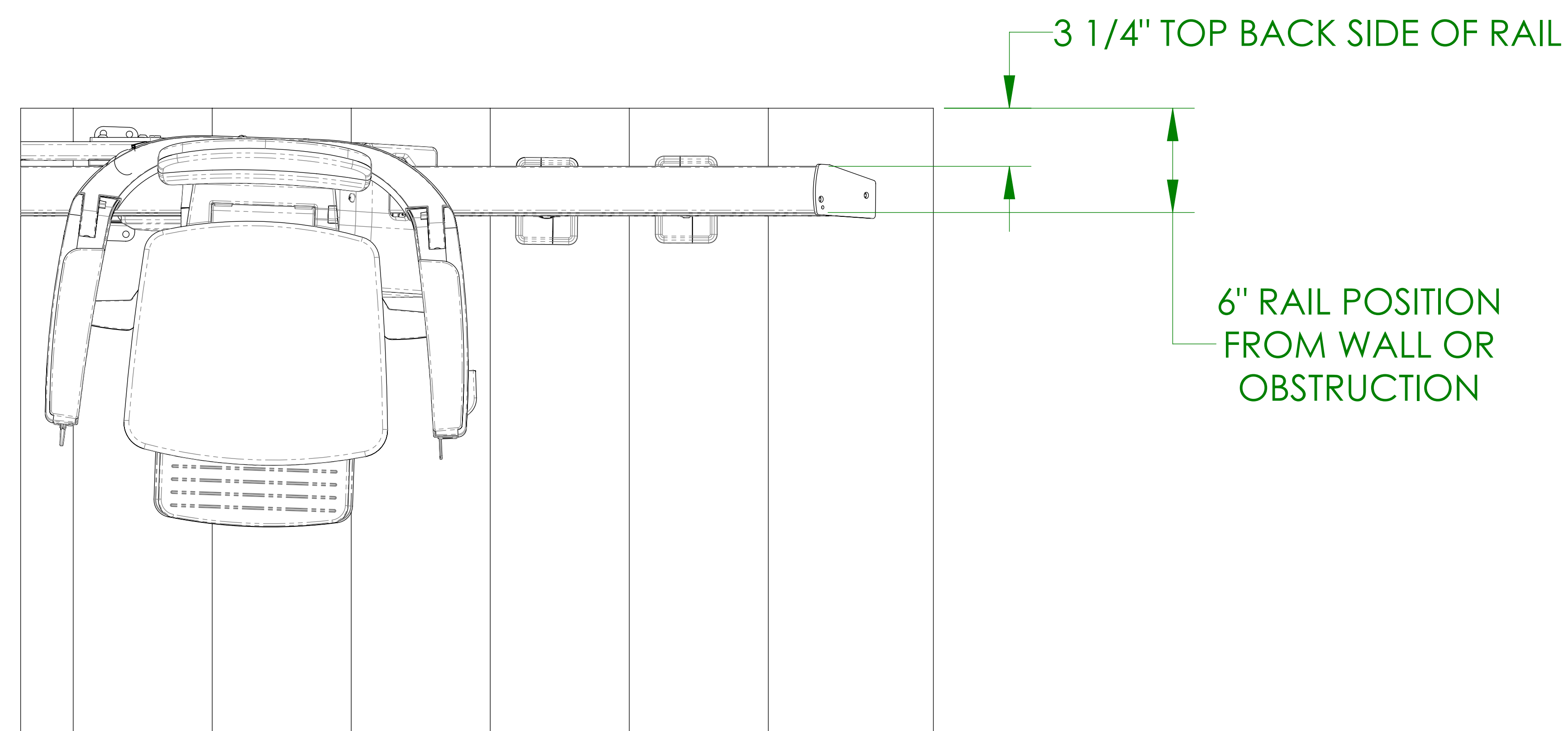
TOP VIEW
