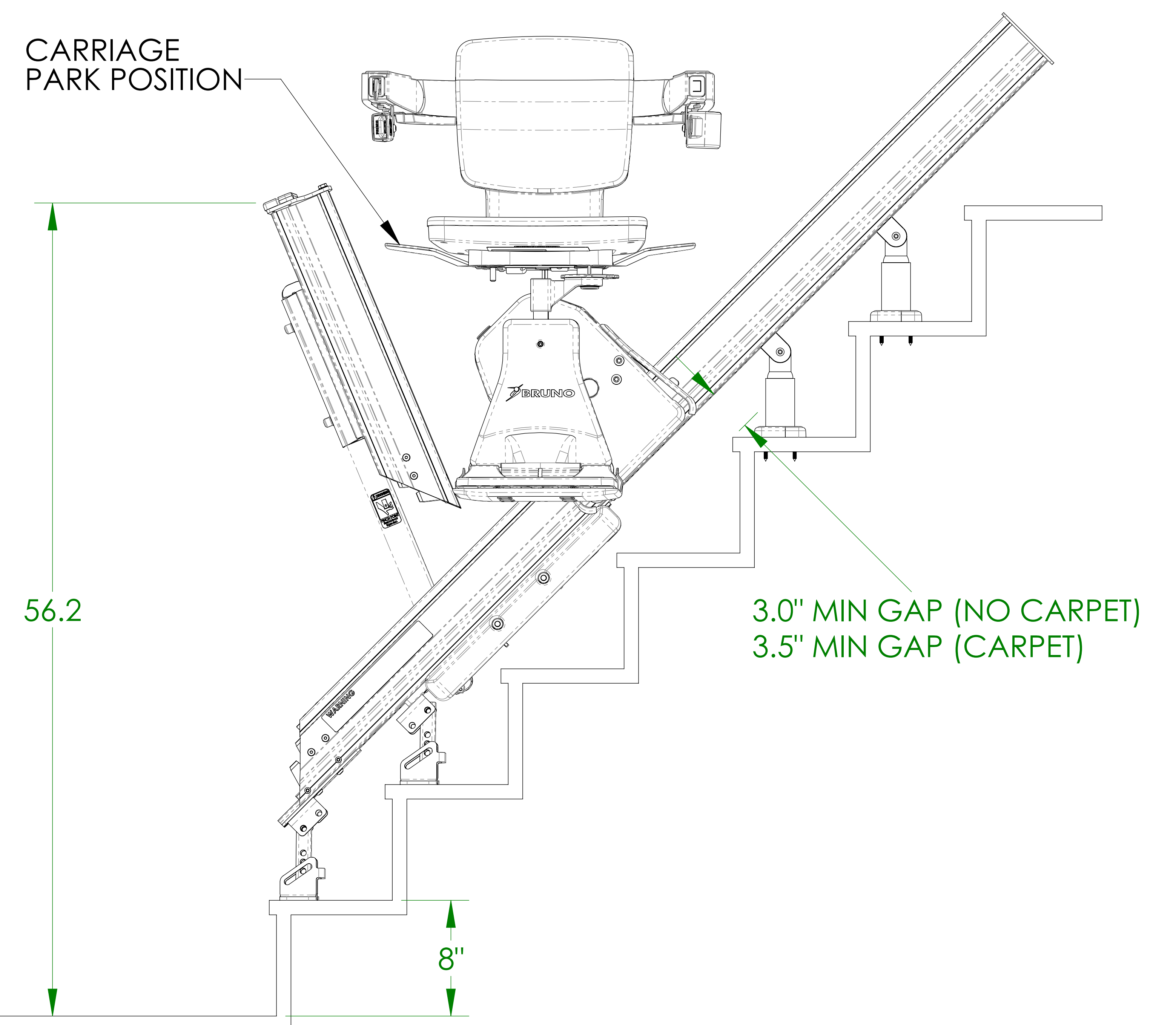
AUXILIARY ELEVATION VIEW RAIL FOLDED UP POSITION
